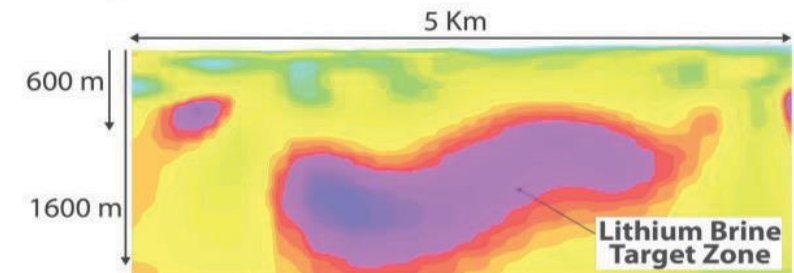
Magnetotellurics Profile
